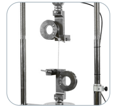
Tensile test on steel wires
