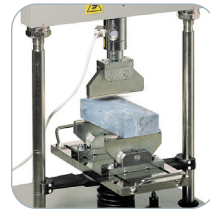
Modulus of rupture of natural building stones
